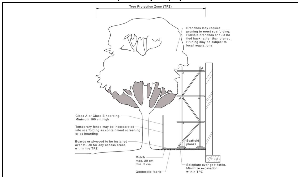
An image from AS4970-2025, with example scaffolding and hoarding.
